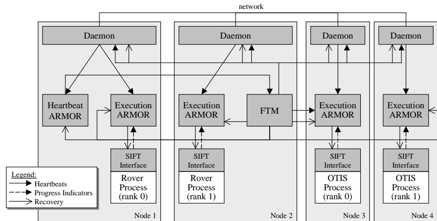
Figure 3: SIFT architecture for executing two MPI applications on a four-node network.
