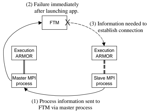
Figure 8: Slave MPI process blocks because Execution ARMOR cannot get information from failed FTM
