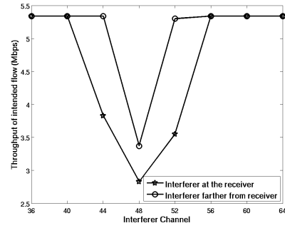
Figure 6. Interference measurements using Senao cards (Tx-Rx distance = 20ft, Main flow channel = 48).
