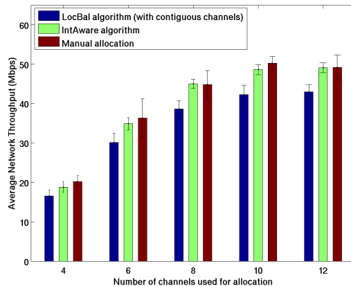
Figure 10. Comparison between the LOCBAL and INTAWARE algorithms - one transmission and one reception at each node.
